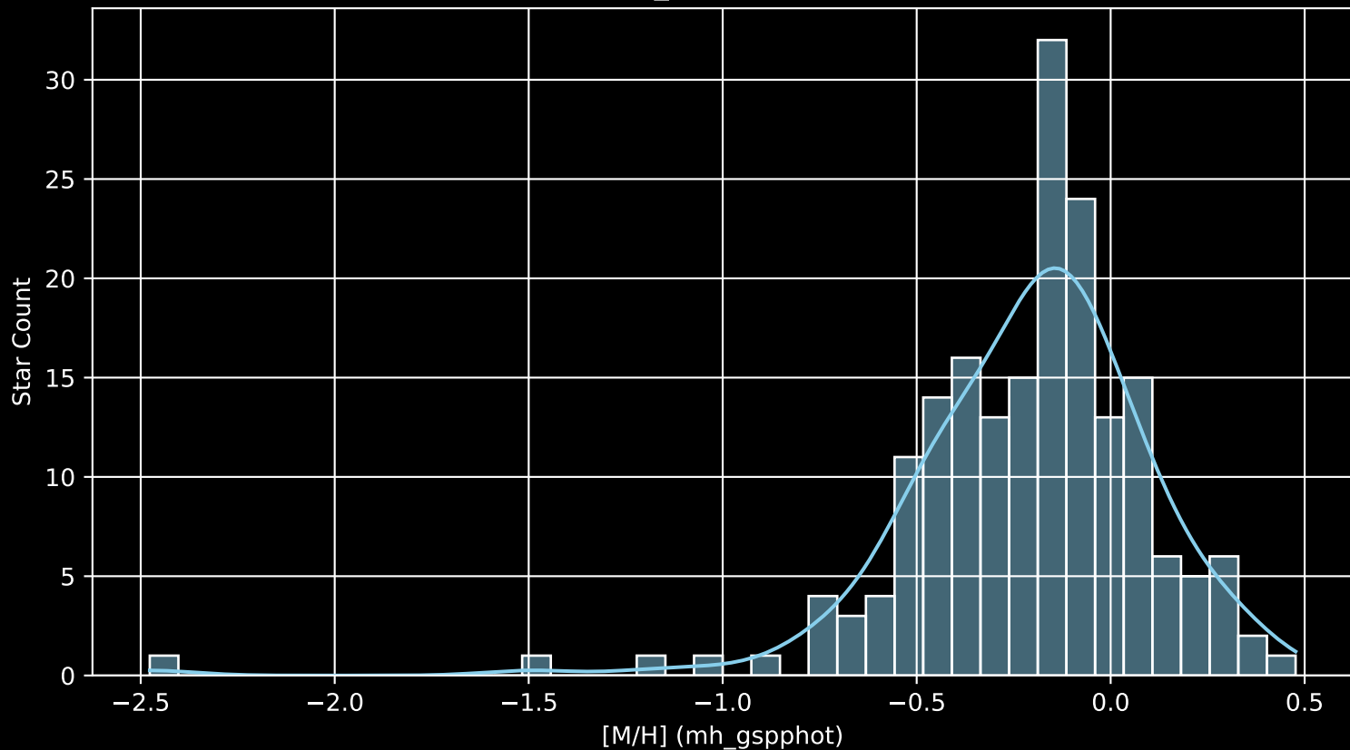
APOGEE DR17 Field: [188+58_MGA [M/H] (mh_gspphot) (n= 189)
