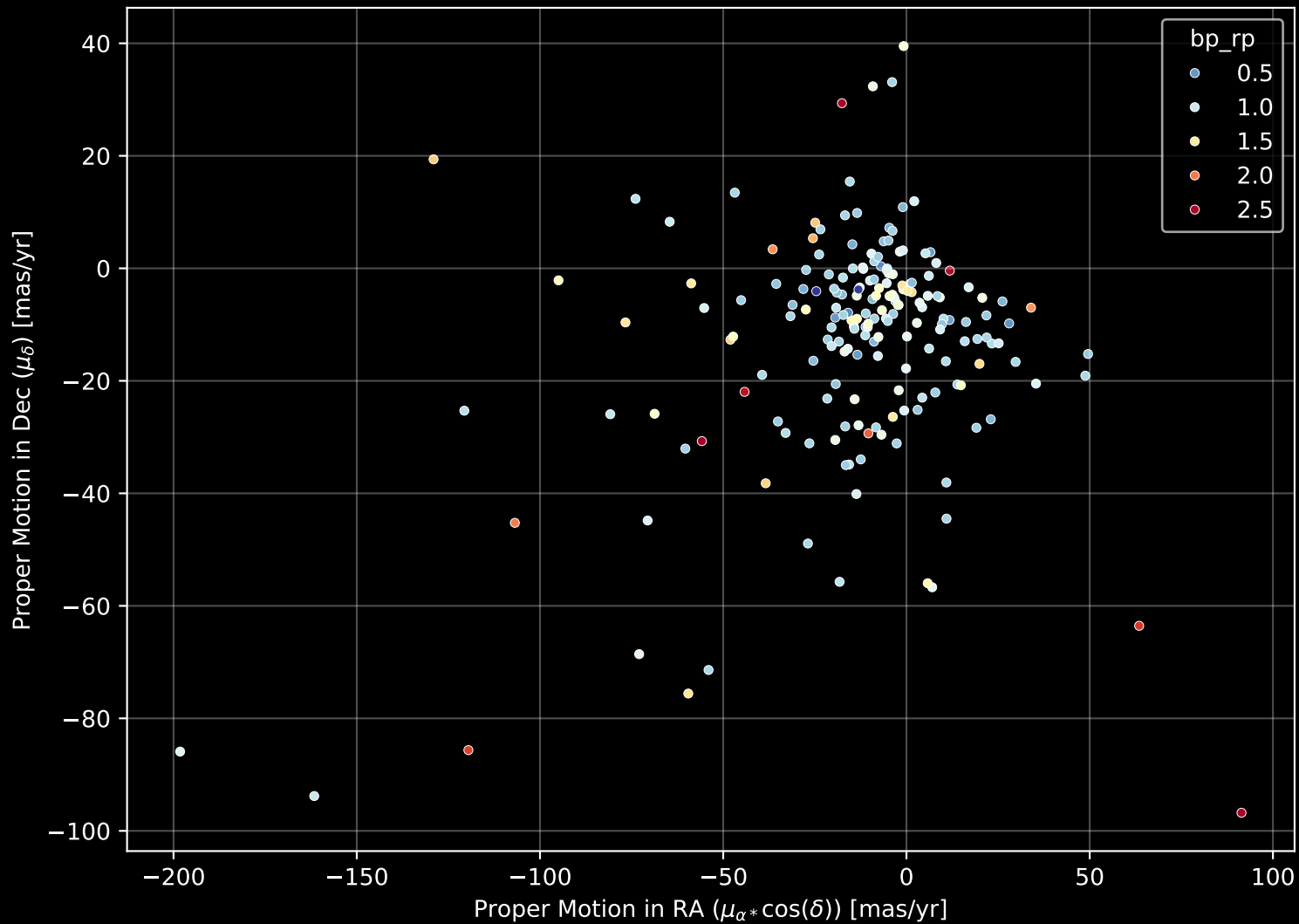
APOGEE DR17 Field: [188+58_MGA] Proper Motion Diagram (n= 192)
