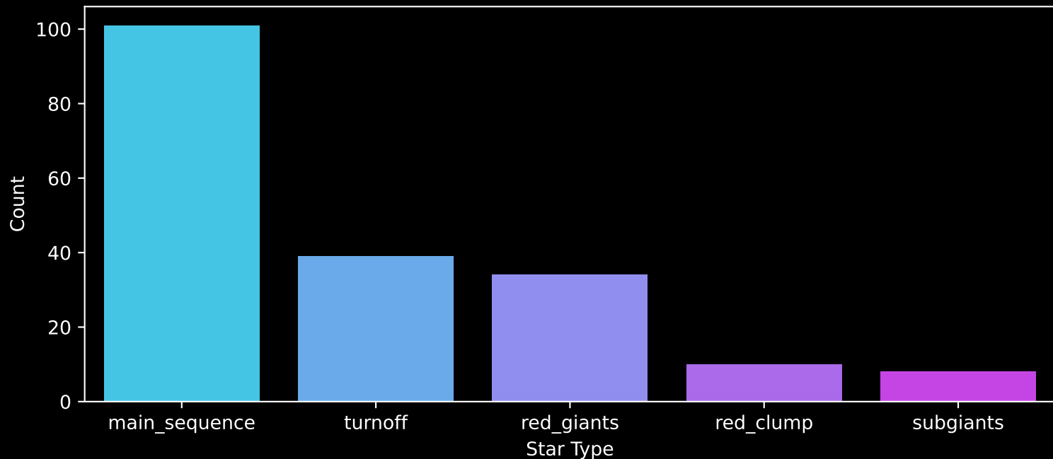
APOGEE DR17 Field: [188+58_MGA] Count plot of Star Type
