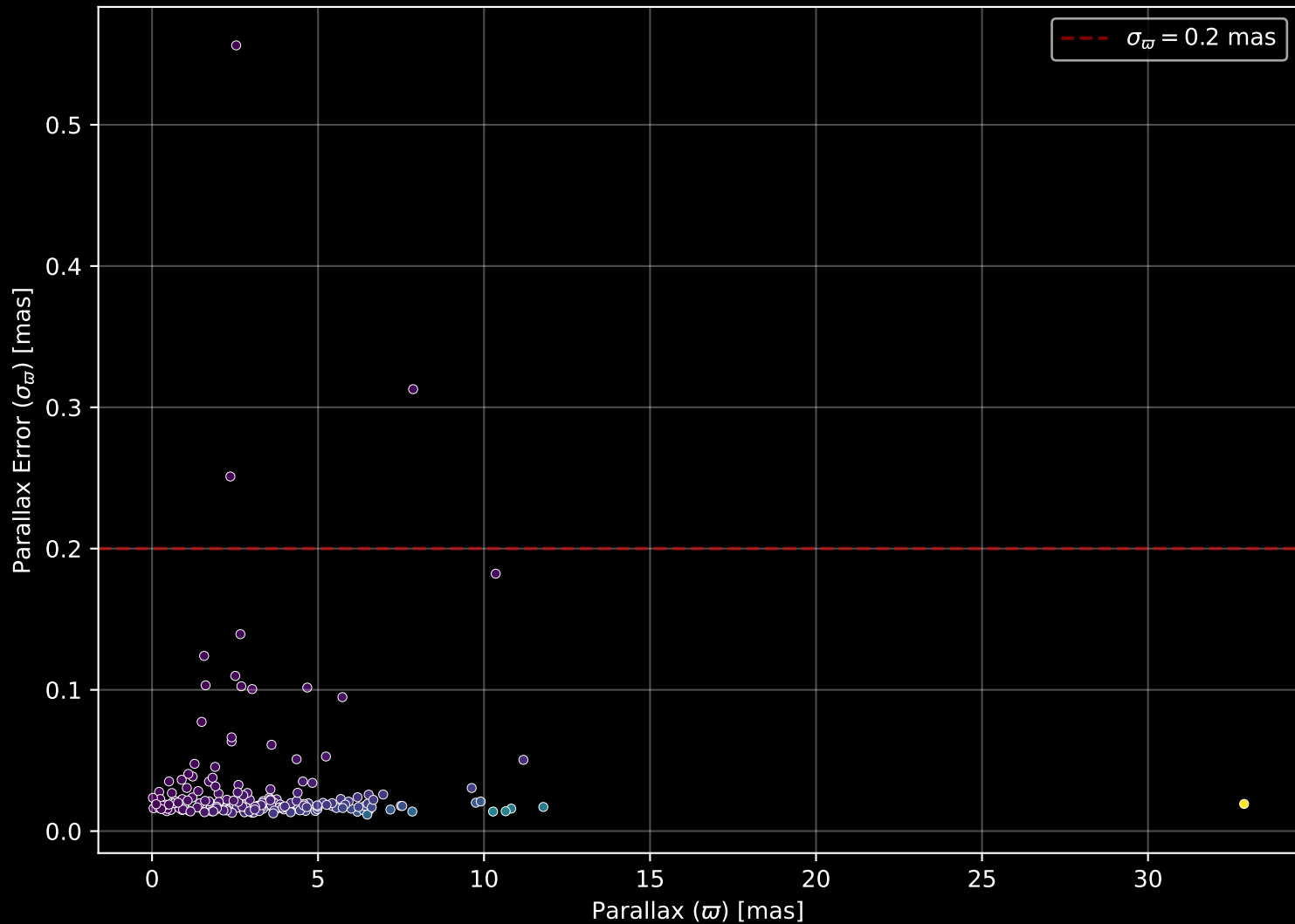
APOGEE DR17 Field: [188+58_MGA] Parallax Quality (n= 192)
